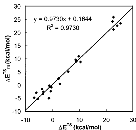
Figure 4. Fitted vs. ab initio values of \Delta E^{TS} for Fit 5 (to compounds 1–22 in the gas phase); the equation of the best-fit line to these data and the correlation coefficient, R^2 , are given
